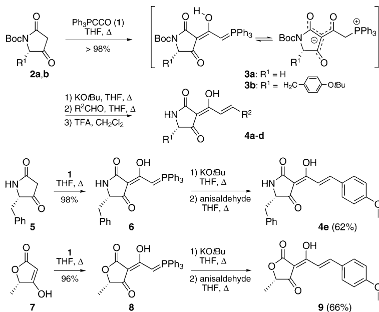
Scheme 1. Selective 3-acylation of tetronic and tetramic acids.
