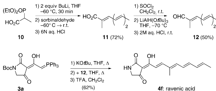
Scheme 2. Synthesis of ravenic acid ( 4f ).
